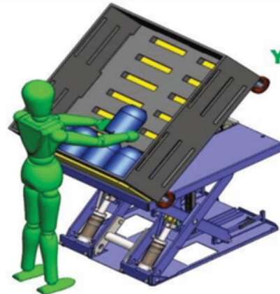
LIFTER & TILTER
